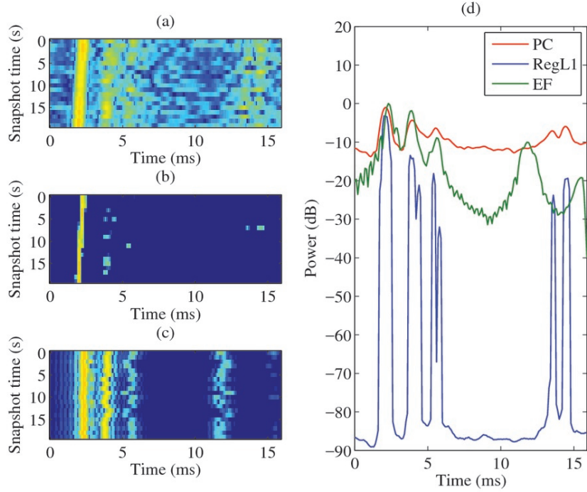
Figure 4.25: Correct CIR alignment, in the sense of an accurate time position of the main path, for the hydrophone 8 data set #274 . Plots (a), (b) and (c) show the CIR in 2D representation for PC, RegL1 and EF, respectively. Plot (d) shows the average magnitude CIR computed with PC (red line), RegL1 (blue line) and EF (green line).
