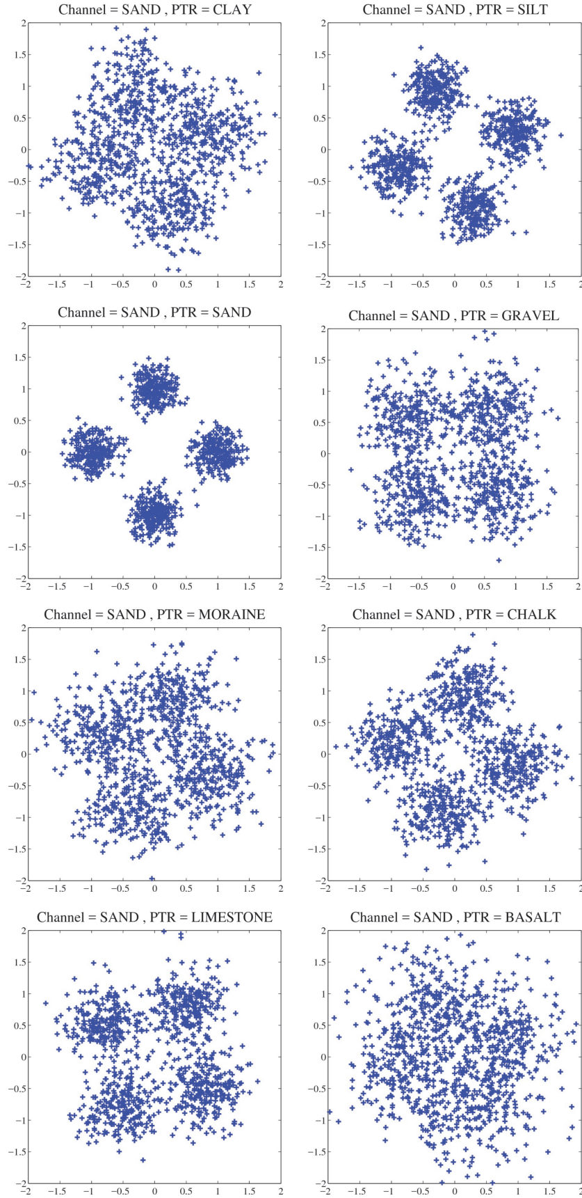
Figure 3.19: Receiver constellations computed in a noiseless channel assuming the mismatch between the reference “actual” CIR from sand bottom and each CIR “estimate” of Fig. 3.18 from the reflection coefficients of Fig. 3.17 for bottom types: clay, silt, sand, gravel, moraine, chalk, limestone and basalt, with properties set according to Table 3.2.
