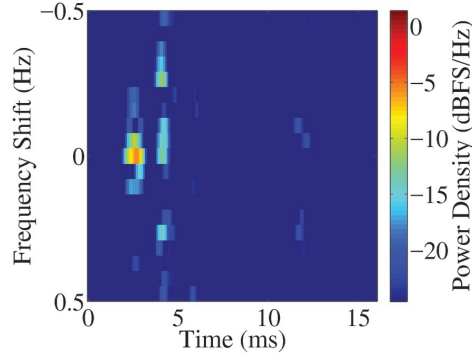
Figure 3.4: Example of DSF computed from the time-variant CIR, generated with 20 snapshot CIR of 16 ms, of Fig. 3.3.
