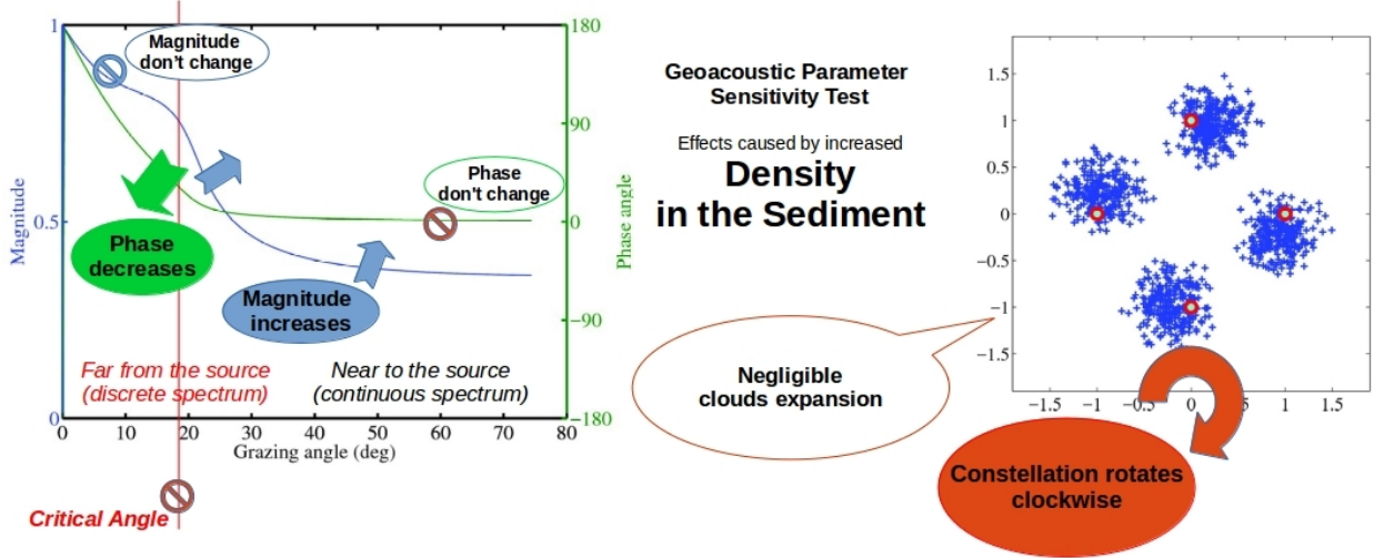
Figure 3.14: Density in sediment layer ( 5m ) over bottom half space testing.
