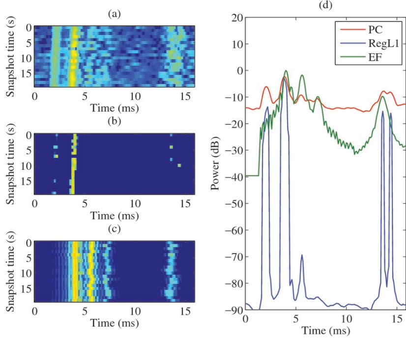
Figure 4.24: Failure in CIR alignment for the hydrophone 8 data set #278 . Plots (a), (b) and (c) show the CIR in 2D representation for PC, RegL1 and EF, respectively. Plot (d) shows the average magnitude CIR computed with PC (red line), RegL1 (blue line) and EF (green line). The first path of EF channel replica wrongly aligned with the second path of PC channel estimate.
